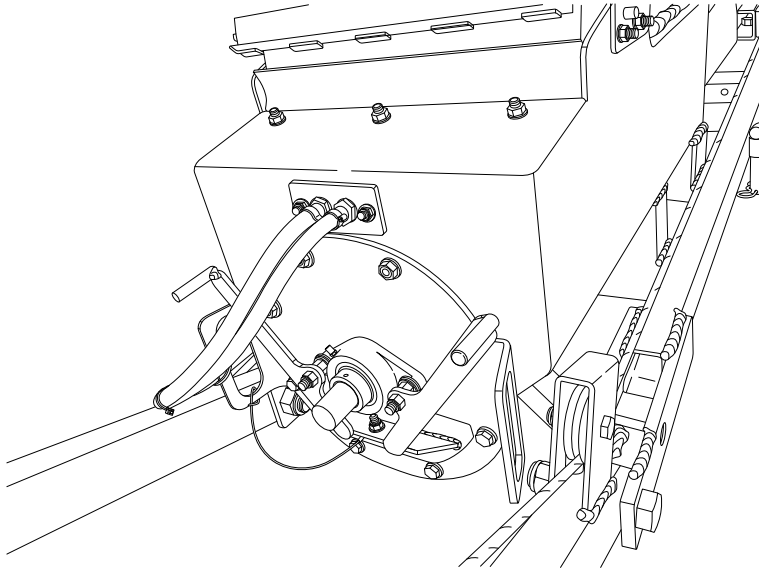
Figure 58. Back Clean-out Door Seal
