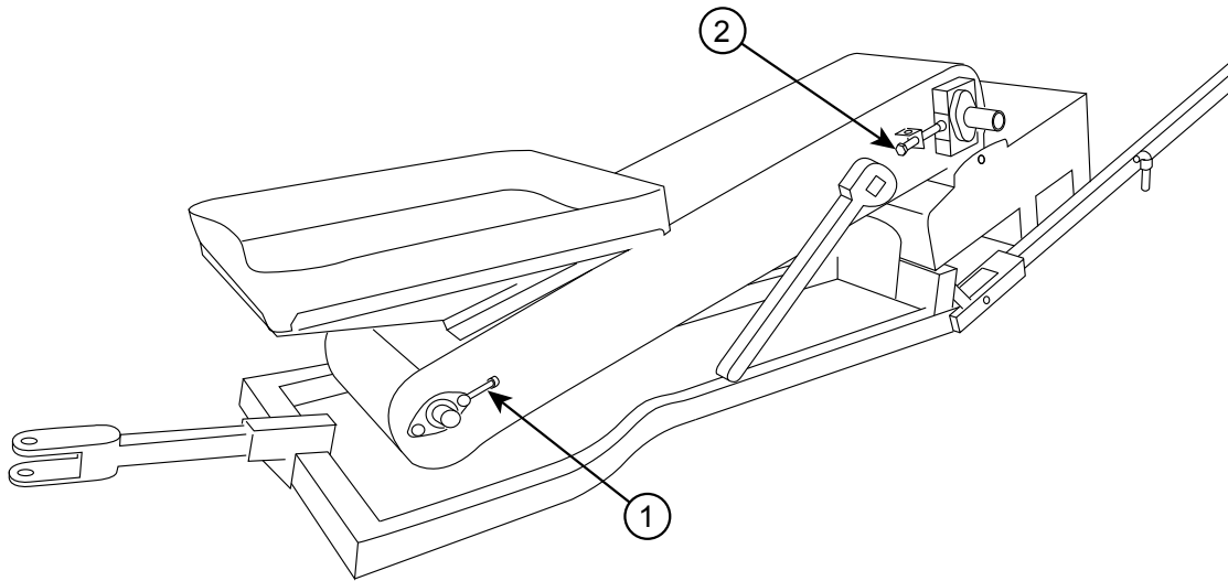
Figure 60. Conveyor Hopper
