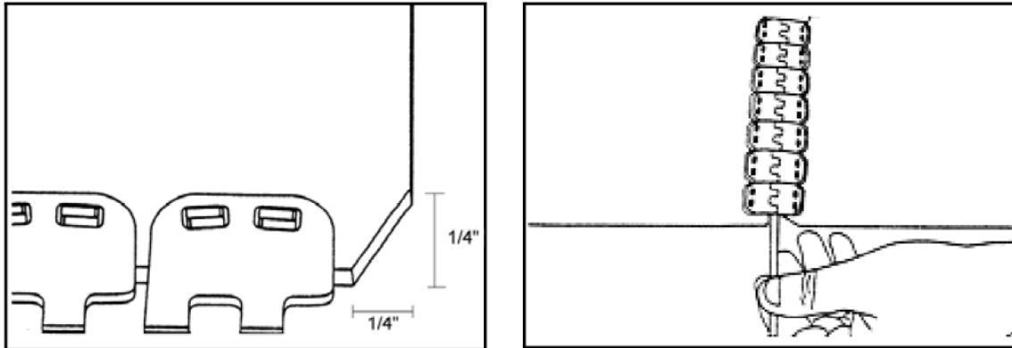
Figure 67. Lacing the Conveyor Belt
