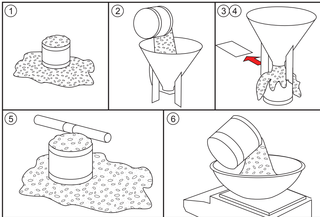
Figure 72. Test Weight Procedure Steps
