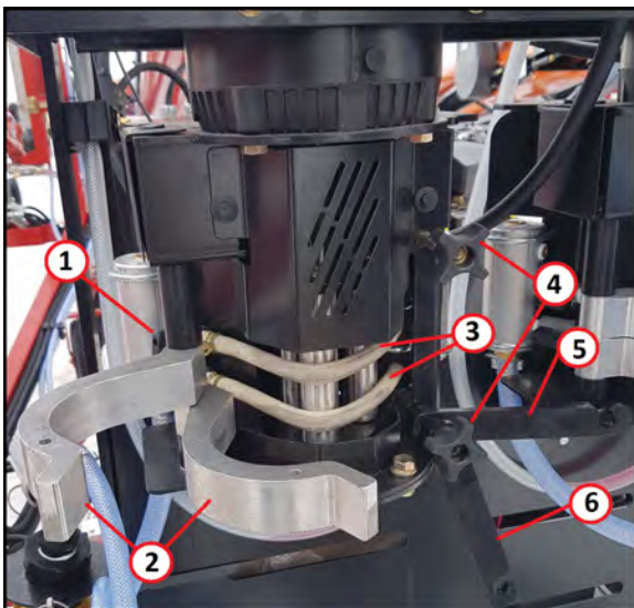
Figure 8. Pump Overview
