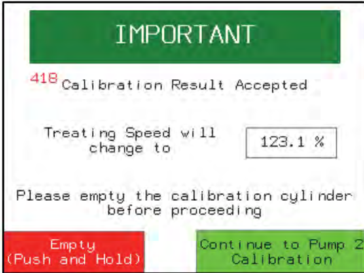
Figure 29. Calibration Outcome Screen
