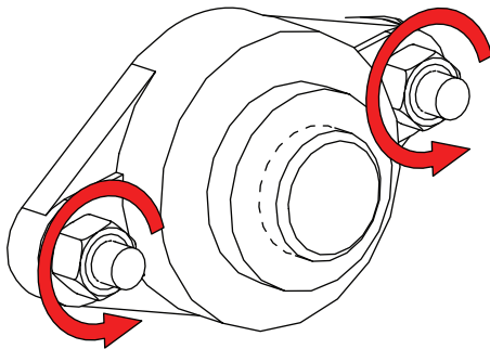
Figure 63. Loosen the Bearing Nuts
