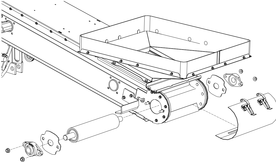
Figure 59. Replacing a Conveyor Roller
