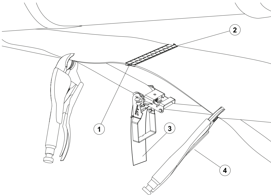
Figure 66. Using the Ratchet Strap
