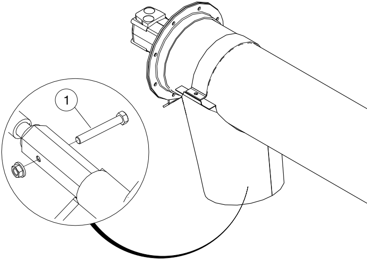
Figure 71. Removing the Shear Bolt
