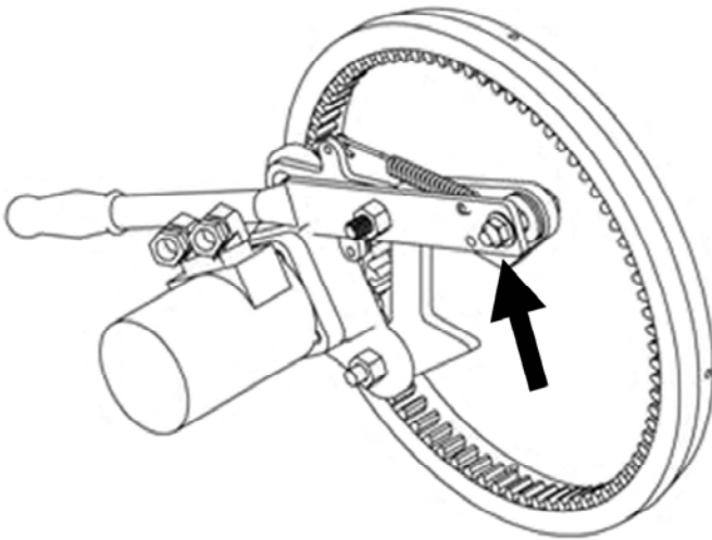
Figure 70. Pinion Gear Adjustment Nut
