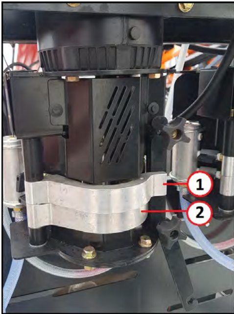
Figure 9. Pump Shoe Engaged and Disengaged Positions
