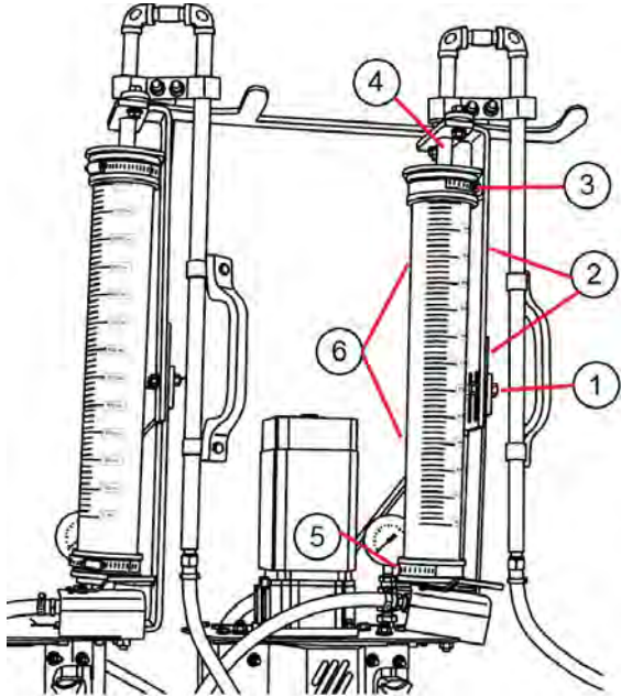
Figure 53. Lubricating the Calibration Chamber
