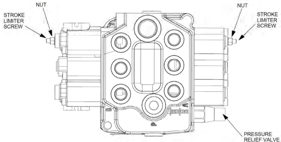
Figure 68. Control Valve Adjustment
