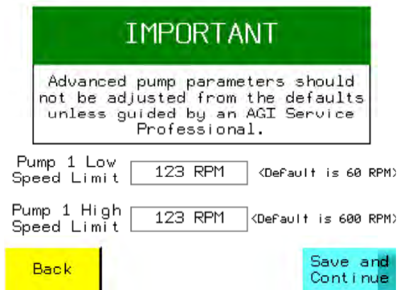
Figure 15. Advanced Pump Setup
