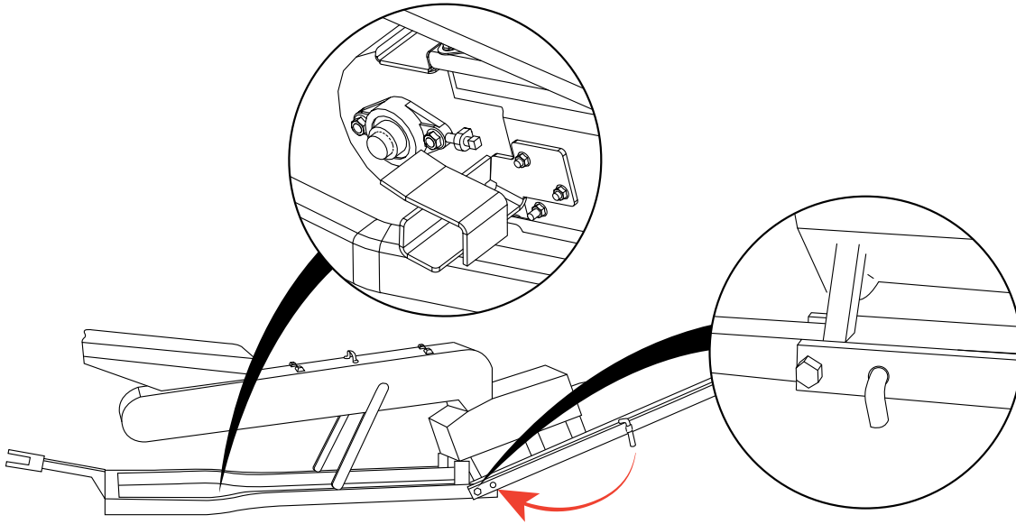
Figure 3. Conveyor Frame and Mover Kit Transport Locks
