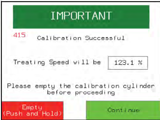
Figure 23. Calibration Successful Outcome Screen
